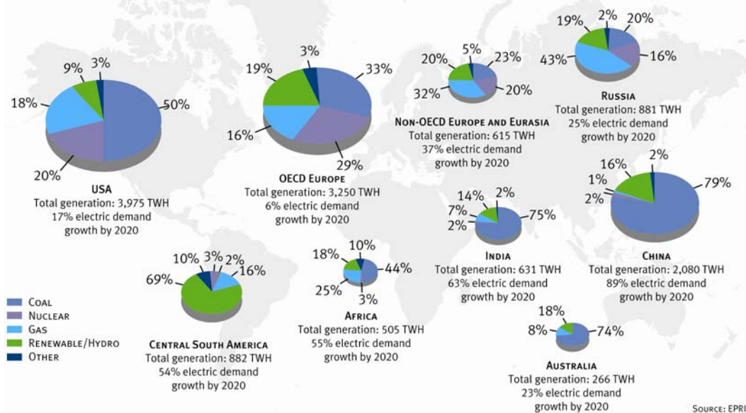
ELECTRICITY GENERATION BY FUEL (2004 & 2020)
