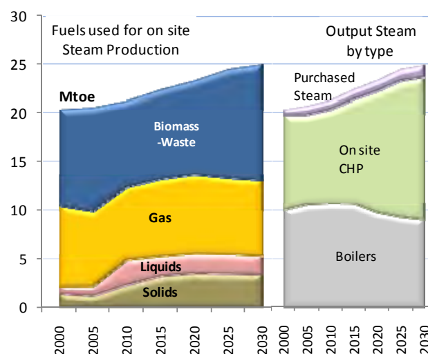
FIGURE 33: STEAM PRODUCTION IN PULP AND PAPER
