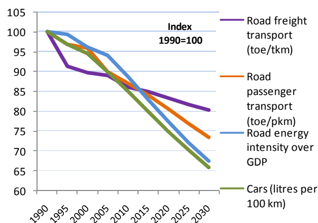
FIGURE 44: ENERGY EFFICIENCY INDICATORS FOR ROAD TRANSPORTATION
