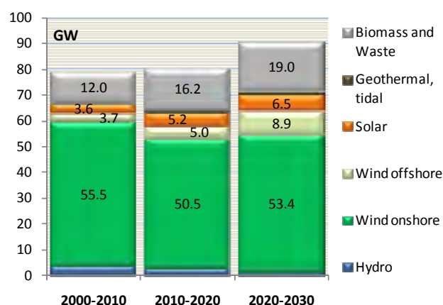
FIGURE 66: INVESTMENT IN RES FOR POWER GENERATION (NET)
