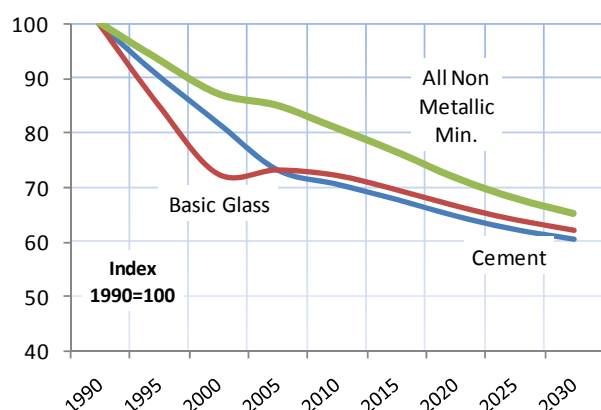
FIGURE 30: ENERGY EFFICIENCY IN NON METALLIC MINERALS
