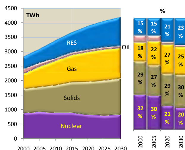
FIGURE 70: POWER GENERATION (NET) BY SOURCE
