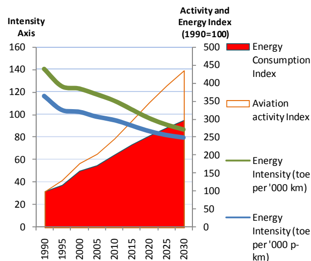
FIGURE 50: ENERGY-RELATED INDICATORS FOR AVIATION
