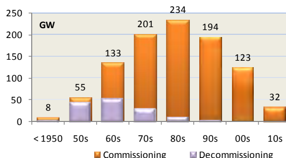
FIGURE 59: DISTRIBUTION OF THERMAL AND NUCLEAR PLANTS BY COMMISSIONING AND DECOMMISSIONING DATE (INFORMATION FROM PRIMES DATABASE)
