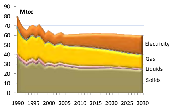
FIGURE 25: ENERGY CONSUMPTION IN IRON AND STEEL
