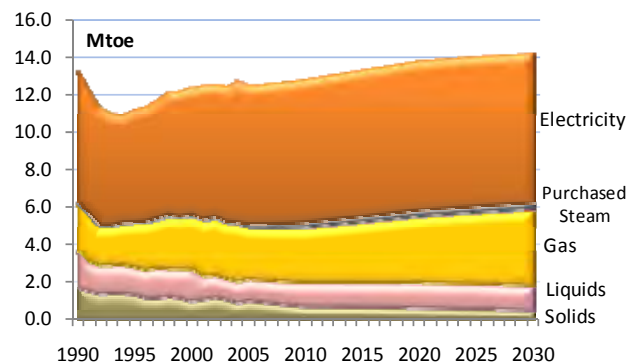
FIGURE 27: ENERGY CONSUMPTION IN NON FERROUS
