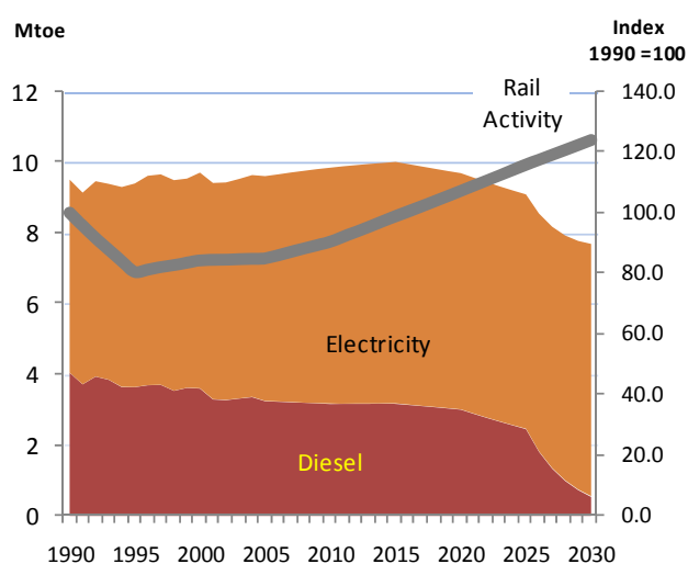
FIGURE 48: ENERGY CONSUMPTION IN RAIL TRANSPORT
