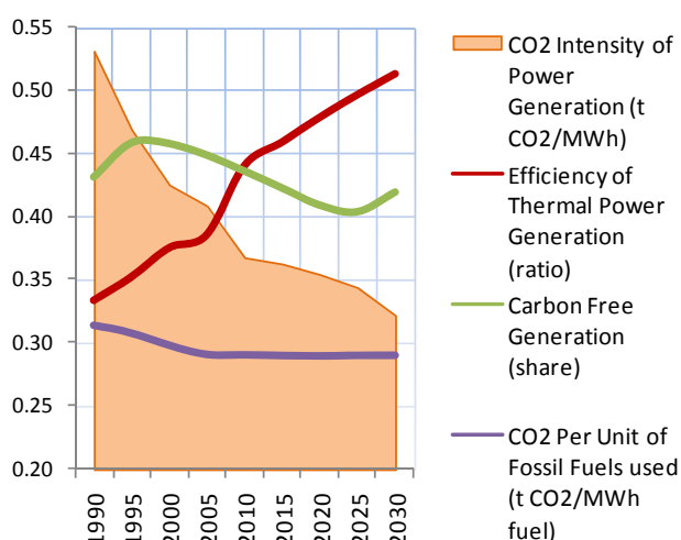
FIGURE 76: CARBON-RELATED INDICATORS
