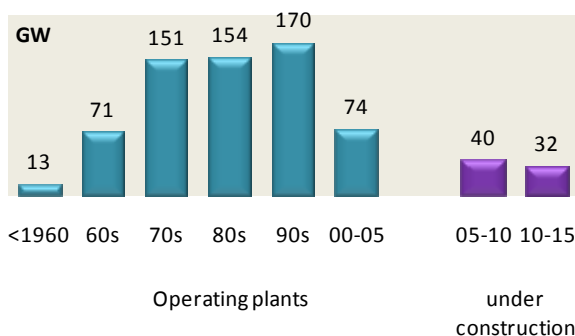
FIGURE 62: DISTRIBUTION OF GAS AND COAL PLANTS
