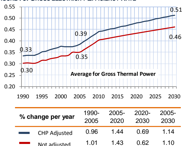
FIGURE 73: GROSS ELECTRICITY EFFICIENCY RATE
