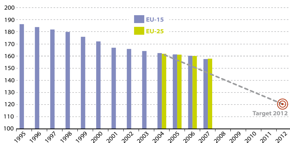
Figure 3.15: Average CO 2 emissions per km from new passenger cars (g CO 2 /km)
